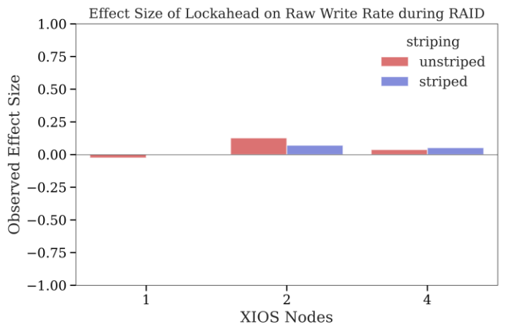
Figure 3. The effect sizes of Lockahead mode between control and RAID periods on raw write rate (GiBs/s) compared to the effect sizes of standard locking mode under the same conditions, grouped by number of Lustre stripes (1 or 2). Values between -0.15 and 0.15 are negligible.
