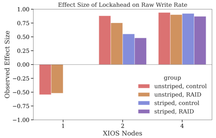
Figure 2. The effect size of Lockahead mode on raw write rate (GiBs/s). Positive values indicate that Lockahead mode caused an increase in raw write rate, and values greater than 0.47 are large.
