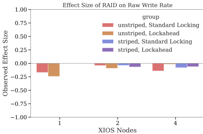
Figure 1. The effect size of RAID checks on raw write rate (GiBs/s). Negative values indicate that RAID checks caused a decrease in raw write rate, though values between -0.15 and 0.15 are negligible.
